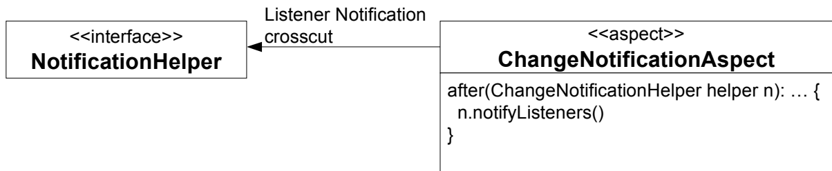
Figure 13. Marker Interface application
